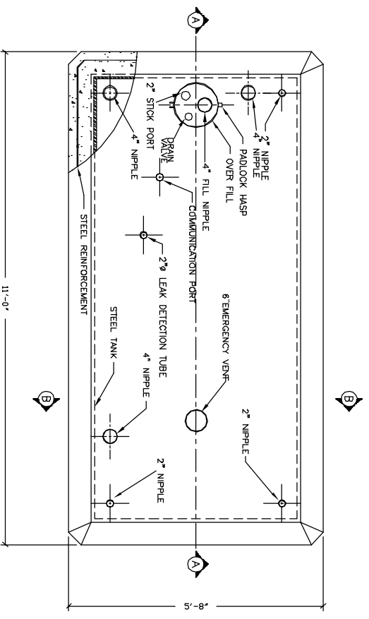
PLAN VIEW
